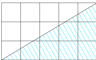
Figure 2: A 3-by-5 rectangle sliced in half to create a triangle of half of the area.
