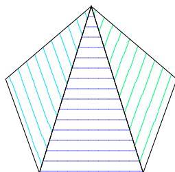
Figure 4: A complex figure (a pentagon), subdivided into figures of known area.
