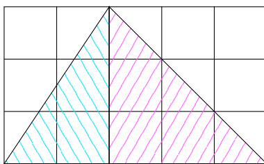
Figure 3: A triangle different from that in Fig. 2 but still of the same base and height.
