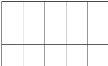
Figure 1: A 3-by-5 rectangle.
